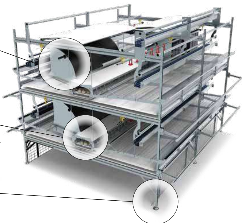
Central egg belt on each tier 290 mm wide
